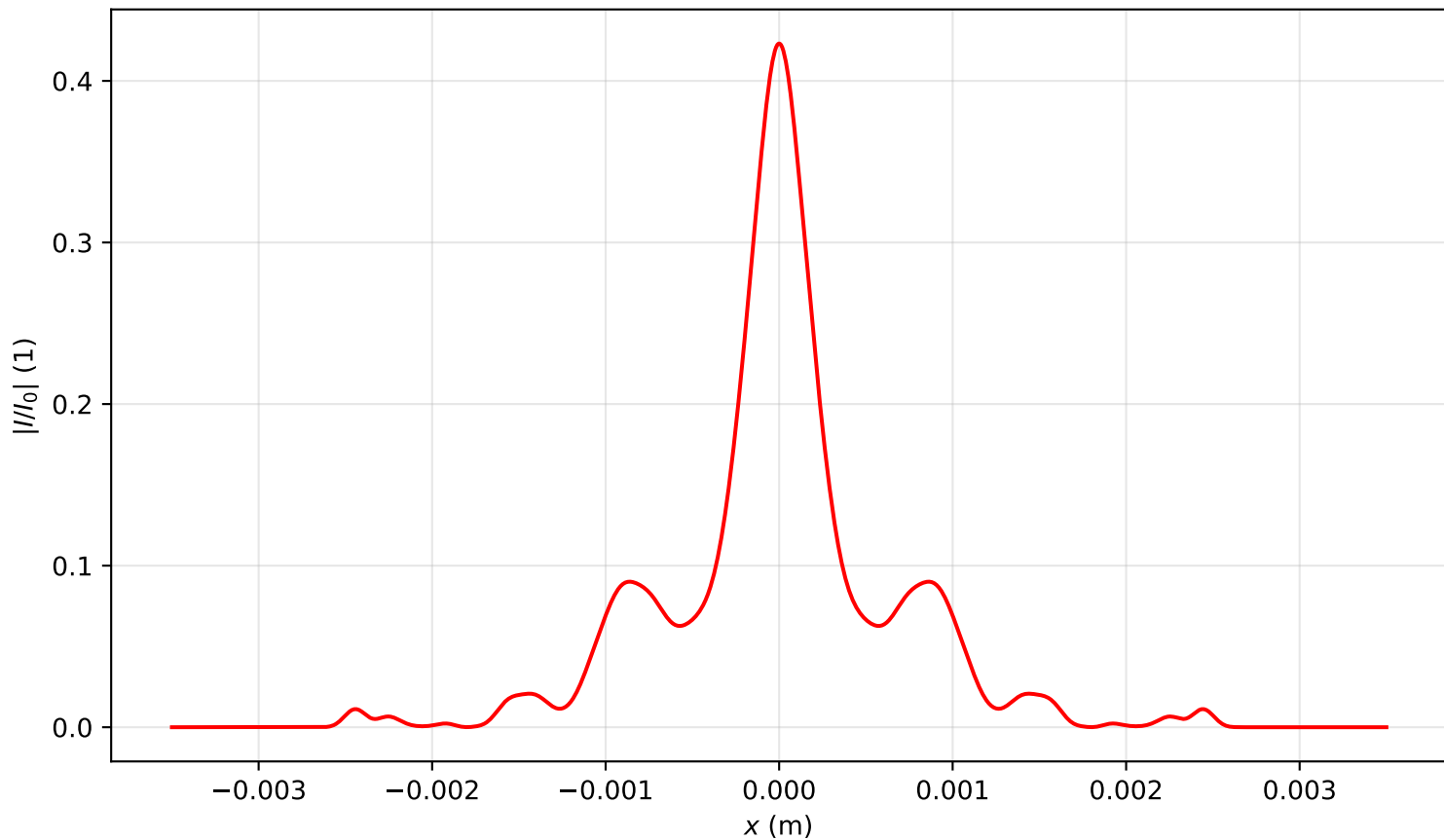
Intensity profile I(x, y = 0, z = 2.388)/I_0 , P_{in}=5.5P_{cr} , artificial time
